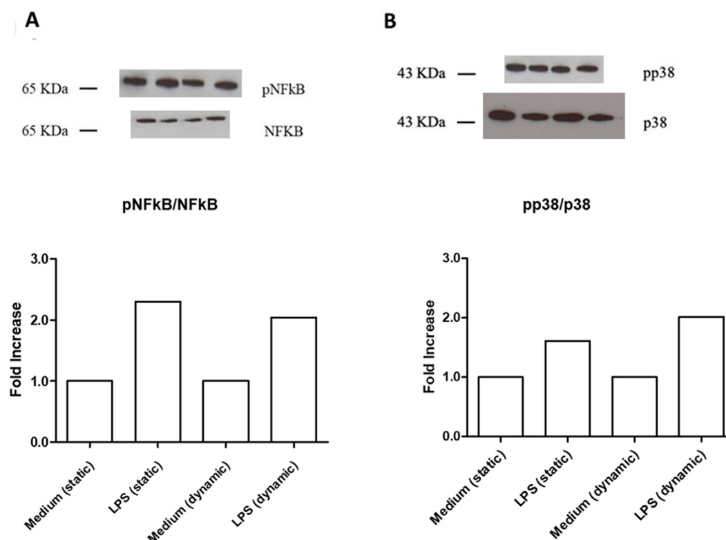
FIGURE 3 Intra-cellular signaling pathways in unstimulated or LPS-stimulated HUVEC seeded in LB1, cultured in static or dynamic conditions. NFκB (A) and p38MAPK (B) phosphorylation after stimulation with LPS (1 μg/mL). Endothelial cells seeded in LB1 for 24 h were incubated with LPS or medium alone both in static and under flow for further 24 h, as experimental control. Results are expressed as the ratio of phosphorylated to non-phosphorylated form, normalized to the respective control and evaluated using Image J software. Western Blotting images are representative of a single experiment. Histograms represent mean of three independent experiments. pNFκB: phosphorylated NFκB; p38MAPK: phosphorylated p38MAPK.
